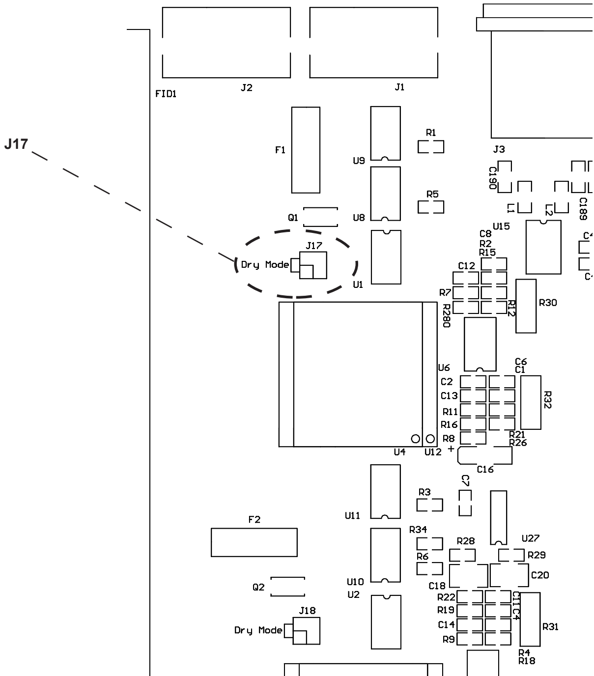
FIGURE 2 - HEADER J17 ON THE DH20 MAIN BOARD
