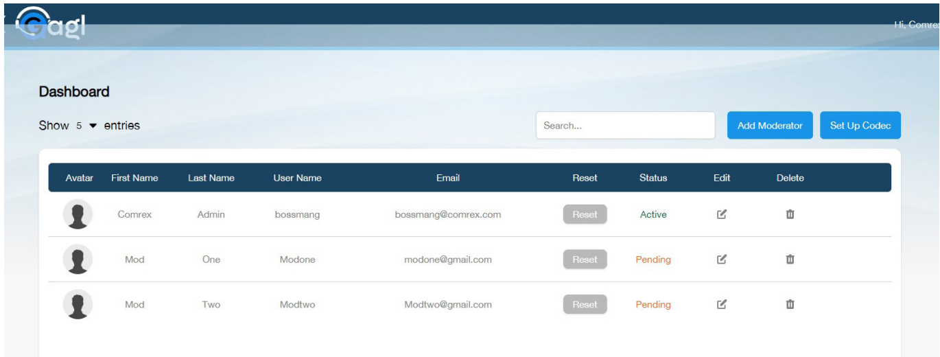
Fig. 3 - Moderator dashboard
